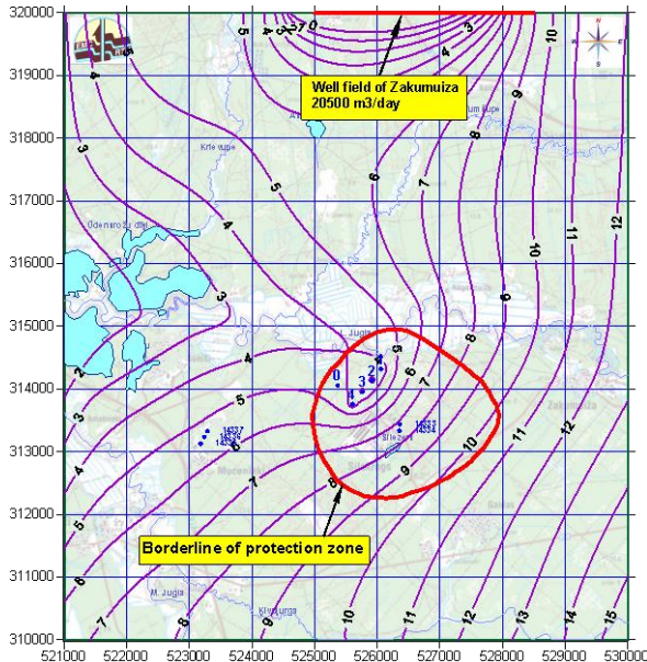
Fig. 6. Head distribution [m asl] of the aquifer D3gj2 if the water production rate is 4000 \text{ m}^3/\text{day} ; the borderline of the chemical protection zone is shown
