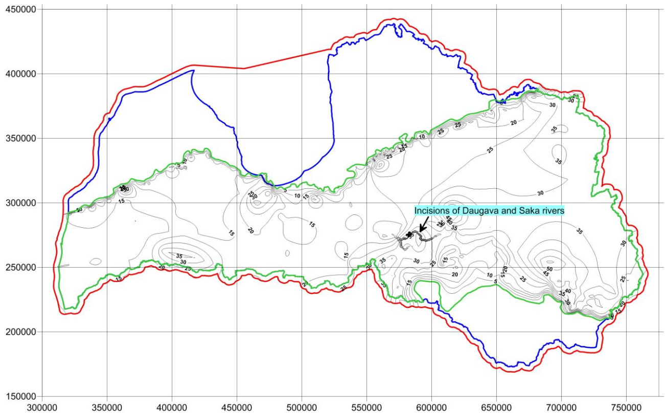
Fig. 3a. M -map for the aquifer thickness; incisions of the Daugava and Saka river valleys.
