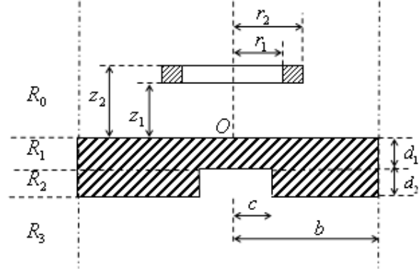
Fig. 3. Coil of finite dimensions above the conducting plate with a cylindrical hole.
