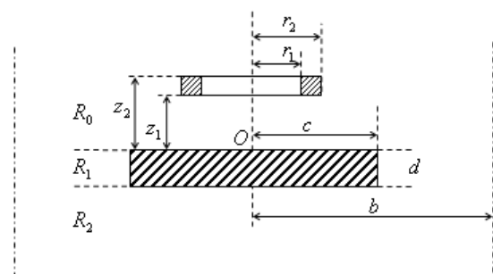
Fig. 1. Coil with alternating current above the conducting cylinder.
