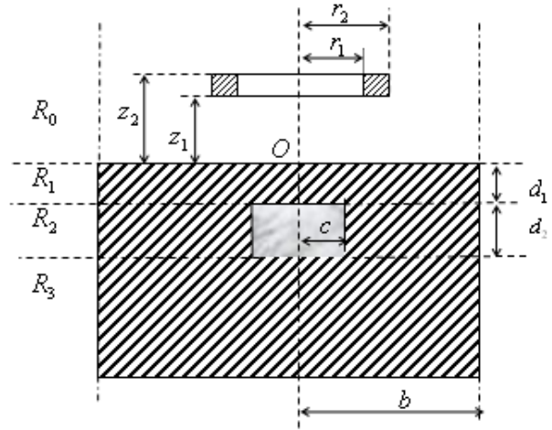
Fig. 4. Coil with finite dimensions above the half-space with a flaw.
