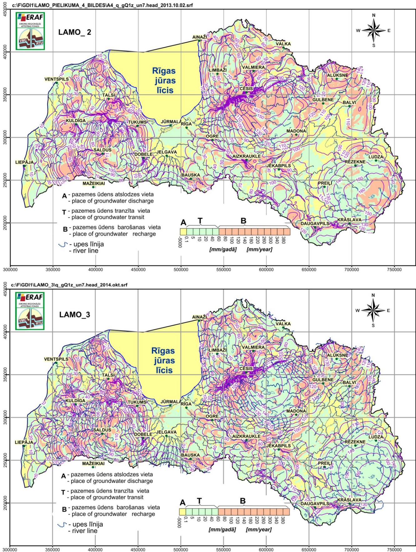
Fig. 2a. Distributions of groundwater flow and heads for primary preQ aquifers of LAMO2 and LAMO3.
