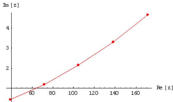
Fig. 5. First five roots of (3).
