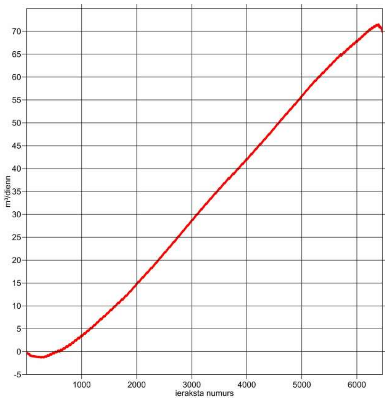
12. att. Ezera pazemes ūdens pietece [ \text{m}^3/\text{dnēn} ]
