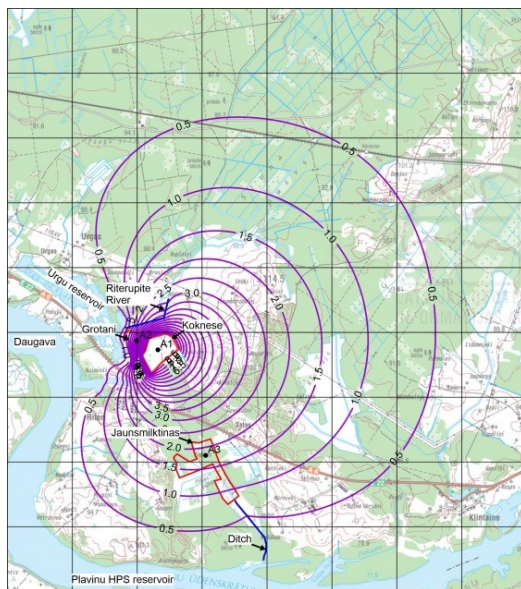
Fig.3. The depression cone isolines [m] for the quarry “Koknese”, S_{A1} = 9.0m
